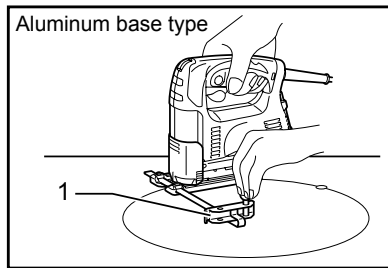
1. Rip fence (Guide rule)
