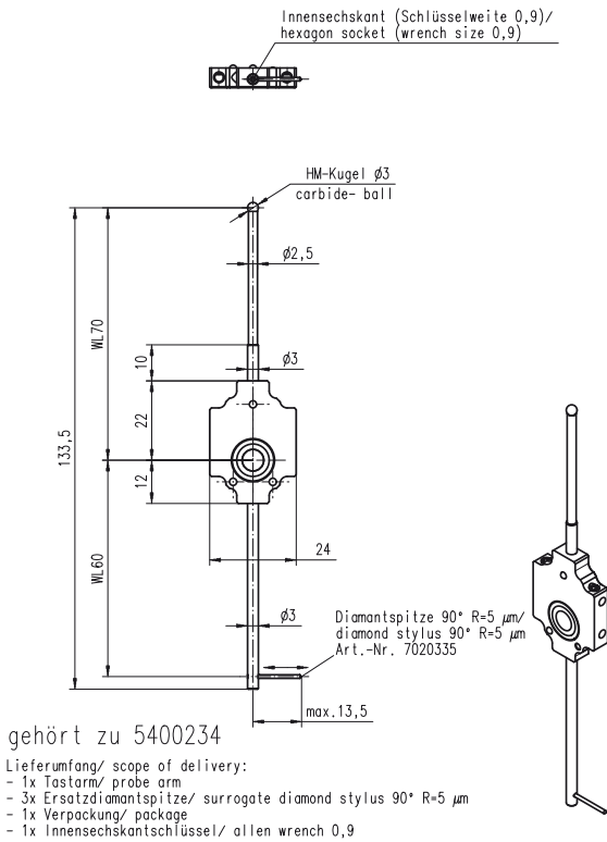
Example of a triple probe arm for form, roughness and contour measuring
