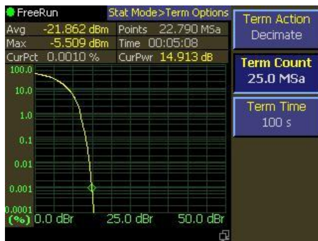
Figure 3-8 CCDF Graphical Display
