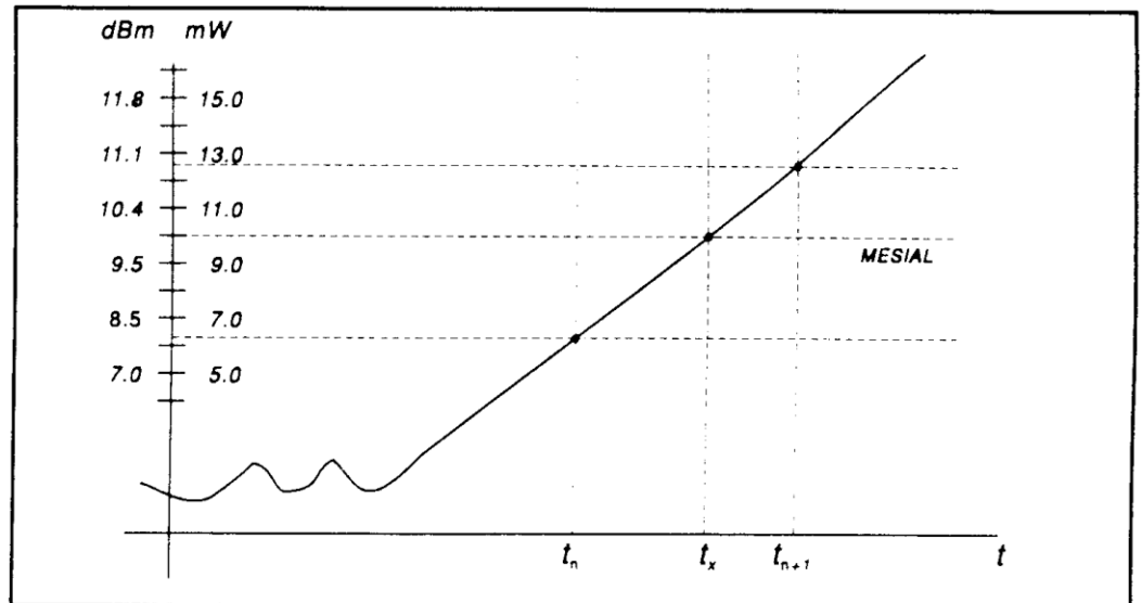
Figure 6-6. Time Interpolation
