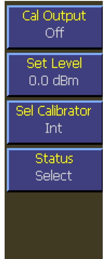
Fig.4-57 Calibrator Menu Internal 50 MHz
