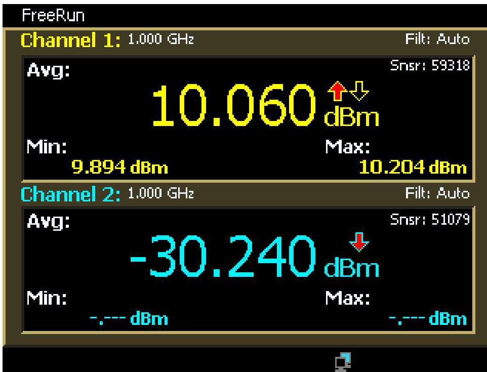
Fig. 4-33A Text Display with Alarm Over-range and Under-range Arrows. (The outline arrow indicates a previous alarm condition that has cleared.)
