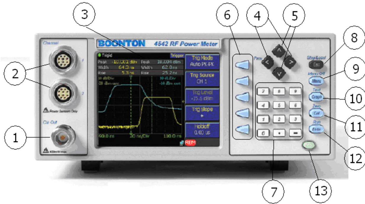
Figure 3-1. Standard 4540 Series RF Power Meter - Front Panel
