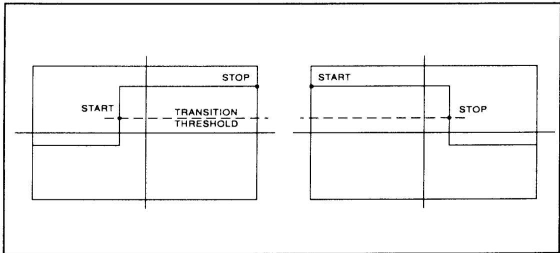
Figure 6-5. Step Waveforms
