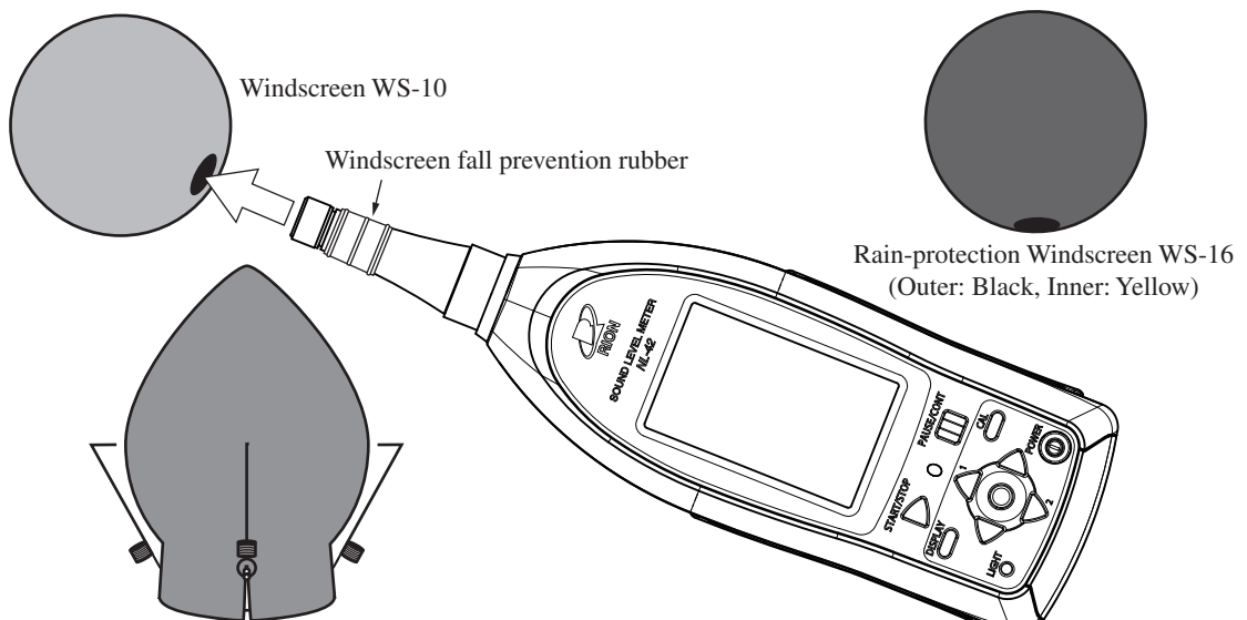
All-Weather Windscreen WS-15
