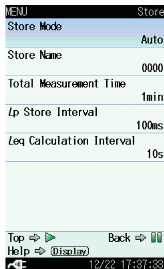
Store screen when Auto mode is selected
